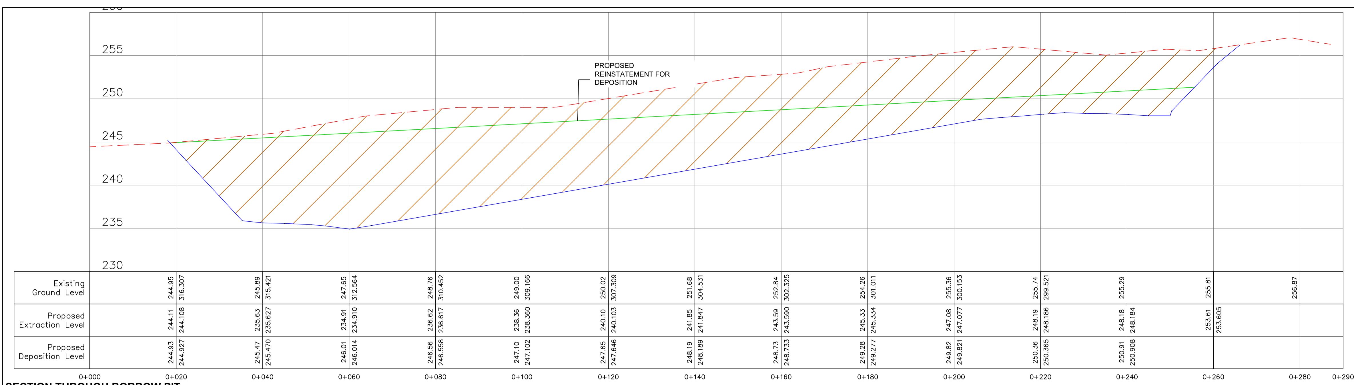
SECTION THROUGH BORROW PIT Scale H- 1:500 / V- 1:250
